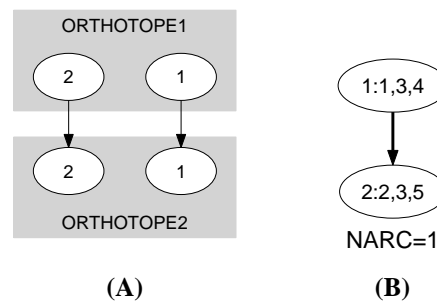
Figure 5.620: Initial and final graph of the two_orth_include constraint
