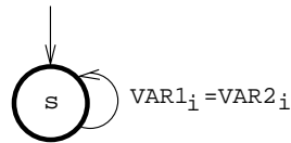
Figure 5.381: Automaton of the lex_equal constraint
