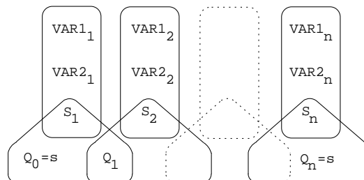
Figure 5.382: Hypergraph of the reformulation corresponding to the automaton of the lex_equal constraint
