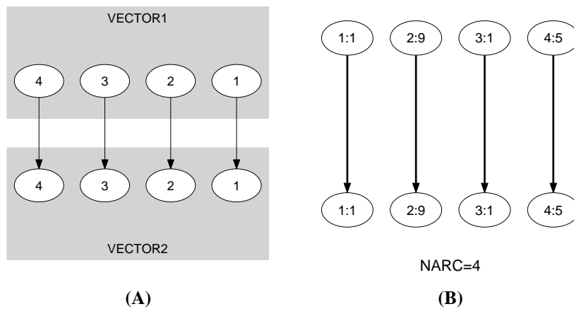
Figure 5.380: Initial and final graph of the lex_equal constraint
