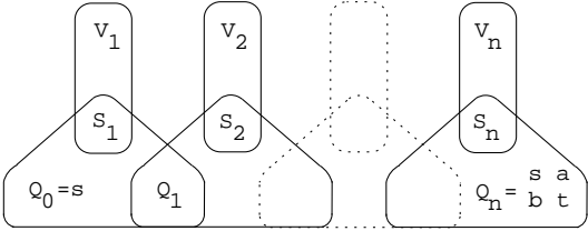
Figure 5.374: Hypergraph of the reformulation corresponding to the automaton of the lex_between constraint
